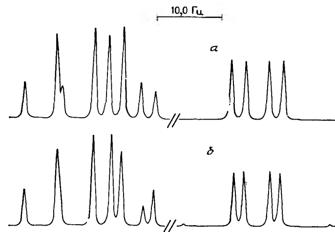
Рис. V. 14. Теоретические ABX-спектры. \alpha - \nu_0(\text{AB}) = 10,0 \text{ Гц}, J_{AB} = 5,0 \text{ Гц}, J_{AX} = 6,0 \text{ Гц}, J_{BX} = 2,0 \text{ Гц}; \beta - \nu_0(\text{AB}) = 10,0 \text{ Гц}, J_{AB} = 5,0 \text{ Гц}, J_{AX} = 6,0 \text{ Гц}, J_{BX} = -2,0 \text{ Гц}.
